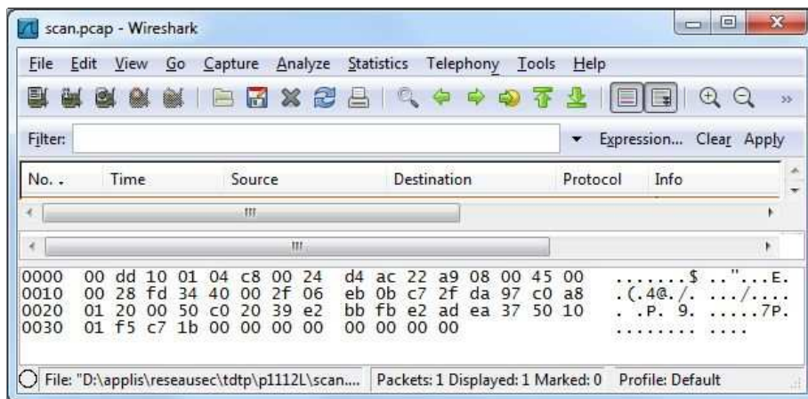
Figure 1: Trame Ethernet
