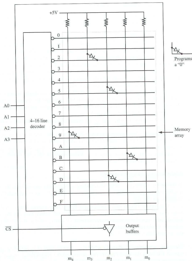
A diode ROM illustrating the n -input address decoder, 2^n \times m memory array, and m output buffers. (From J. Uffenbeck, Microcomputers and Microprocessors: The 8080, 8085, and Z-80 . Prentice Hall, Englewood Cliffs, N.J., 1991.)
